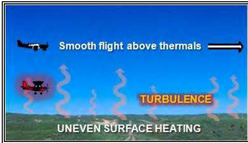
Figure 19-2. Thermals
