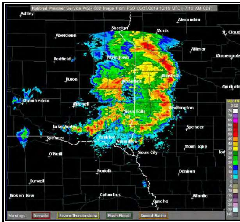
Figure 15-21. WSR-88D Weather Radar Convective Precipitation on the 0.5° Base Reflectivity Product Example
