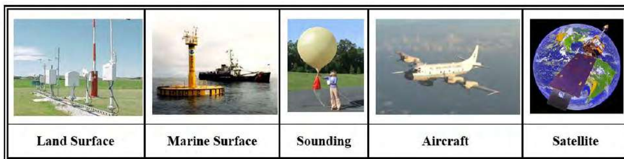
Figure 25-1. Weather Observation Sources
