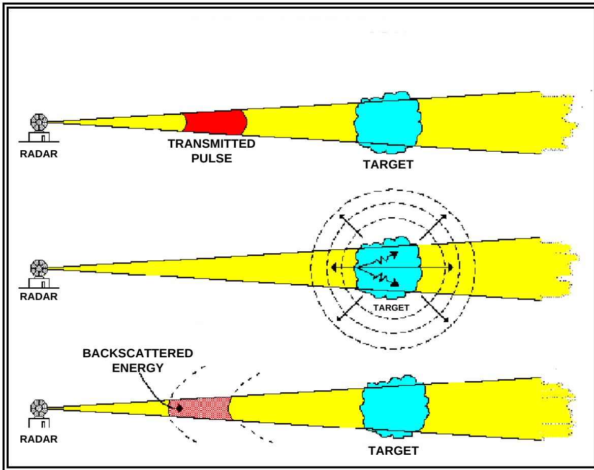
Figure 15-2. Backscattered Energy
