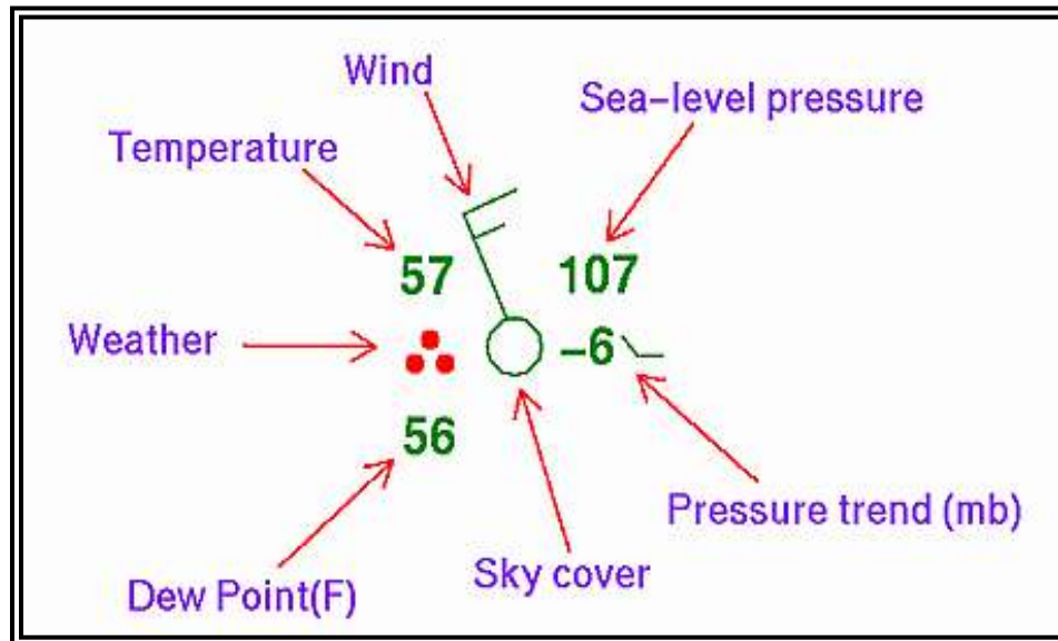
Figure 25-10. NWS Surface Analysis Chart Station Plot Model
