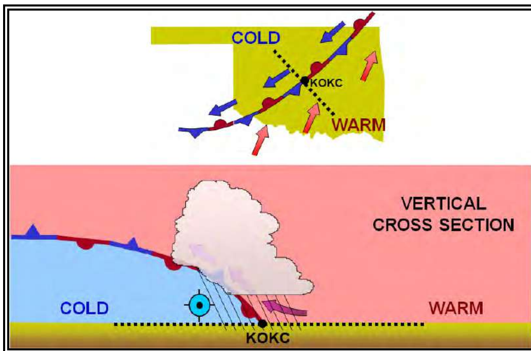
Figure 11-7. Stationary Front
