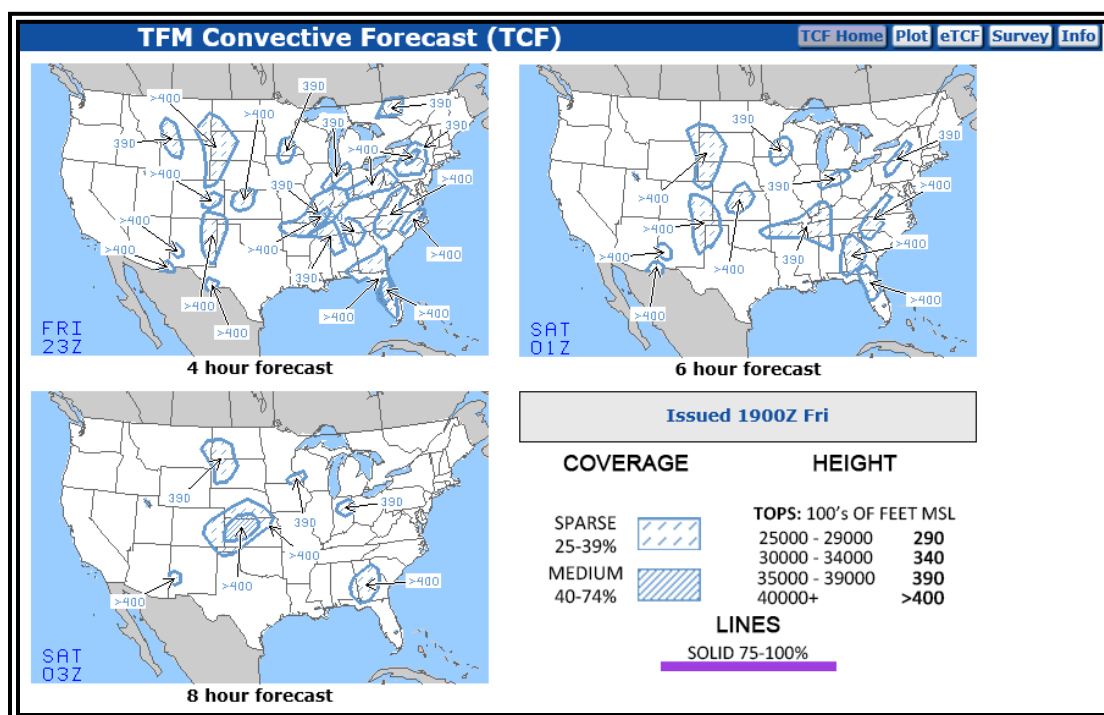
Figure 27-30. TCF Example
