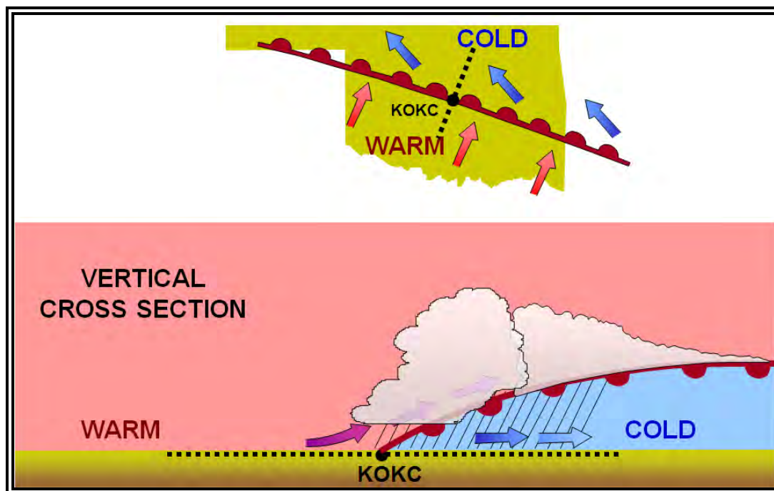
Figure 11-5. Warm Front
