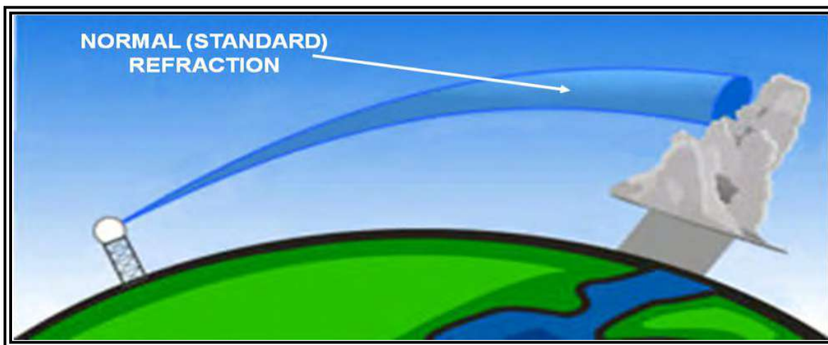
Figure 15-8. Normal Refraction
