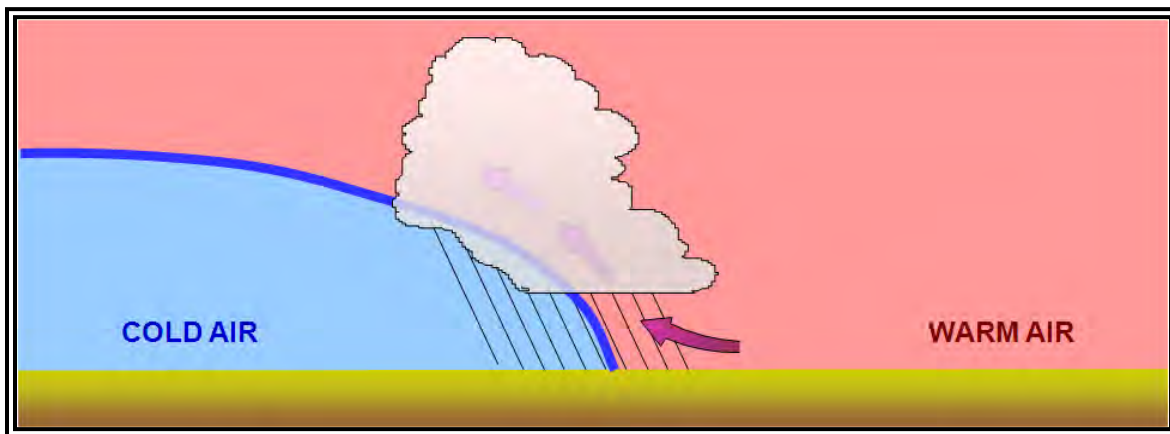
Figure 12-6. Frontal Lift
