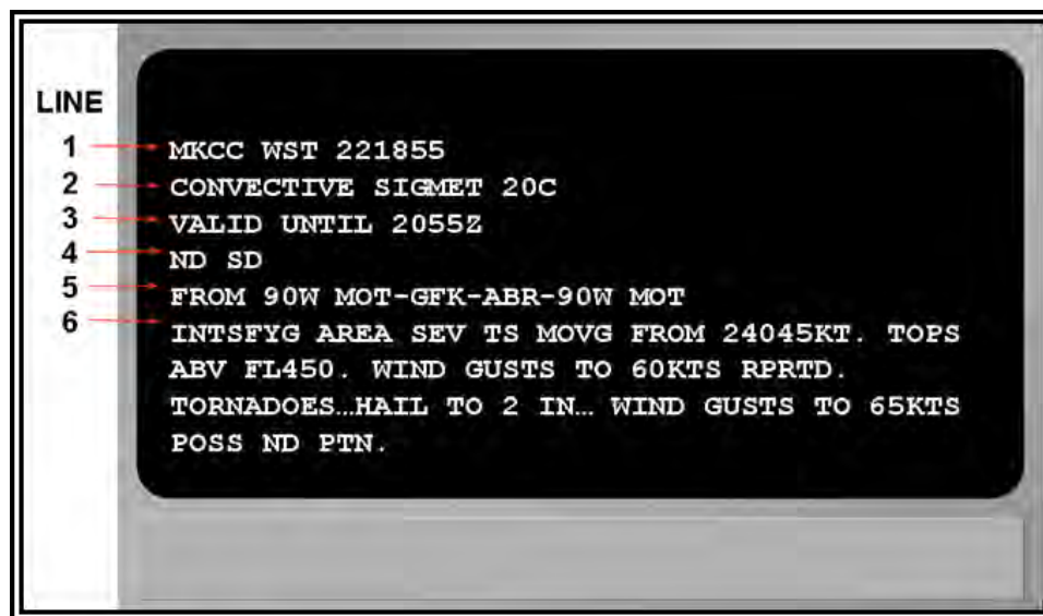
Figure 26-6. Convective SIGMET—Example
