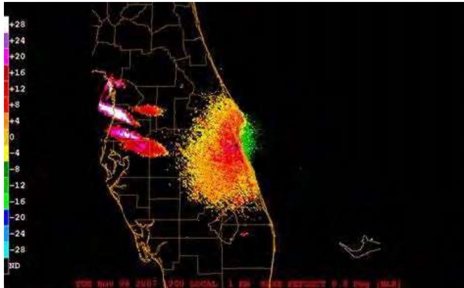
Figure 15-19. Radar Image of Chaff
