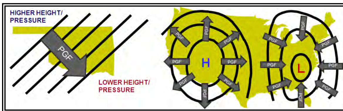
PGF is directed across contours/isobars towards lower height/pressure.
