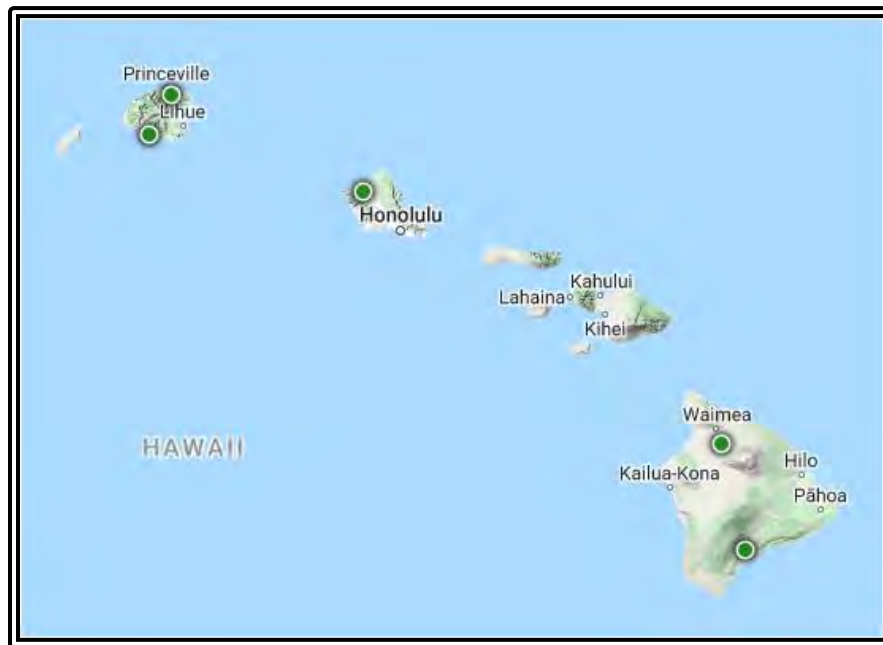
Figure 24-29. Map of the FAA's Aviation Weather Camera Network in Hawaii
