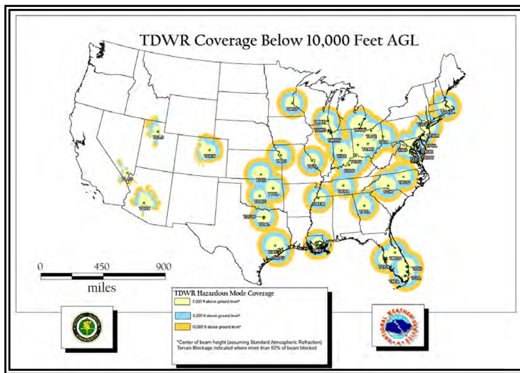
Figure 24-16. TDWR Coverage
