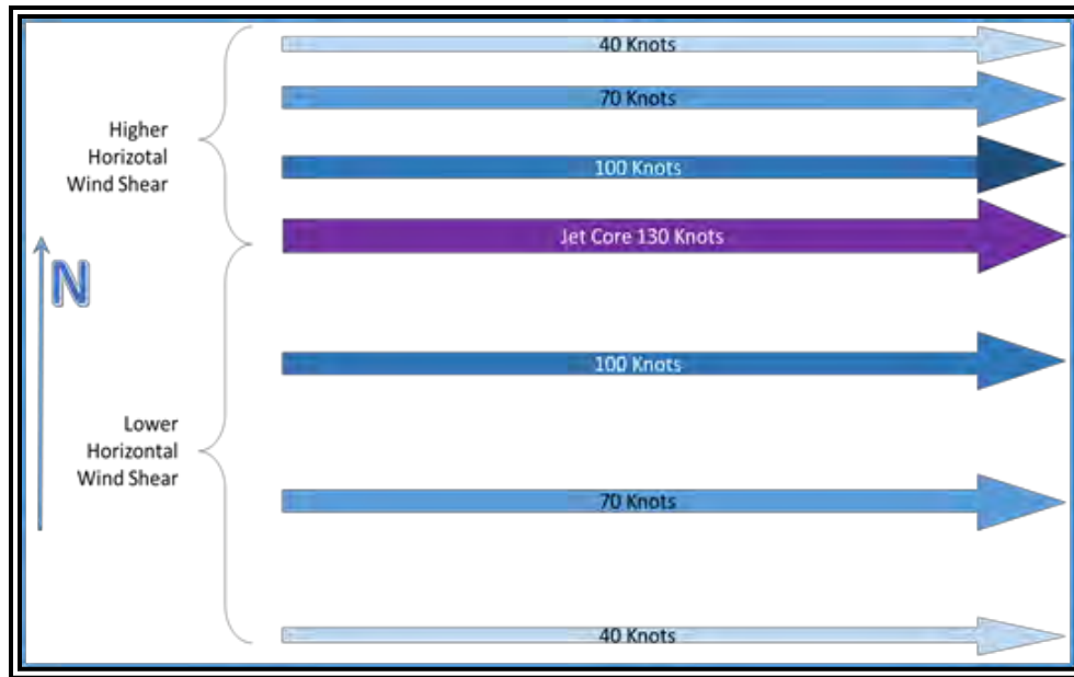
Figure 19-7. Wind Shear Example
