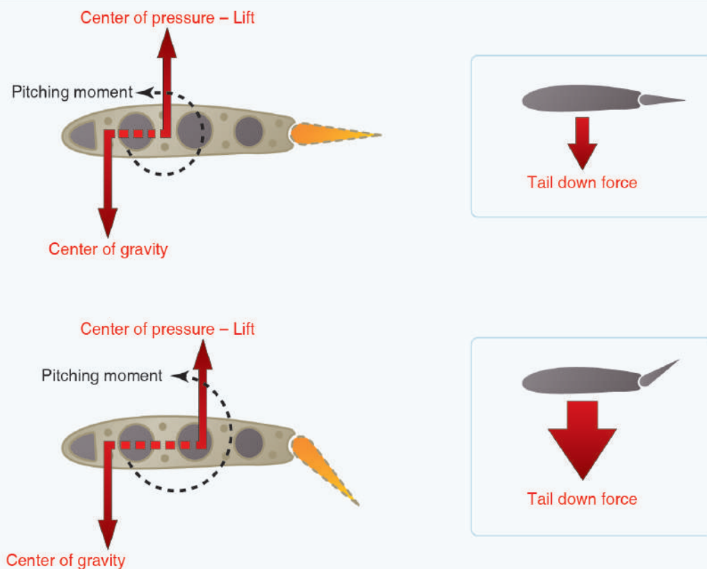
Figure 12-5. Flaps extended pitching moment.
