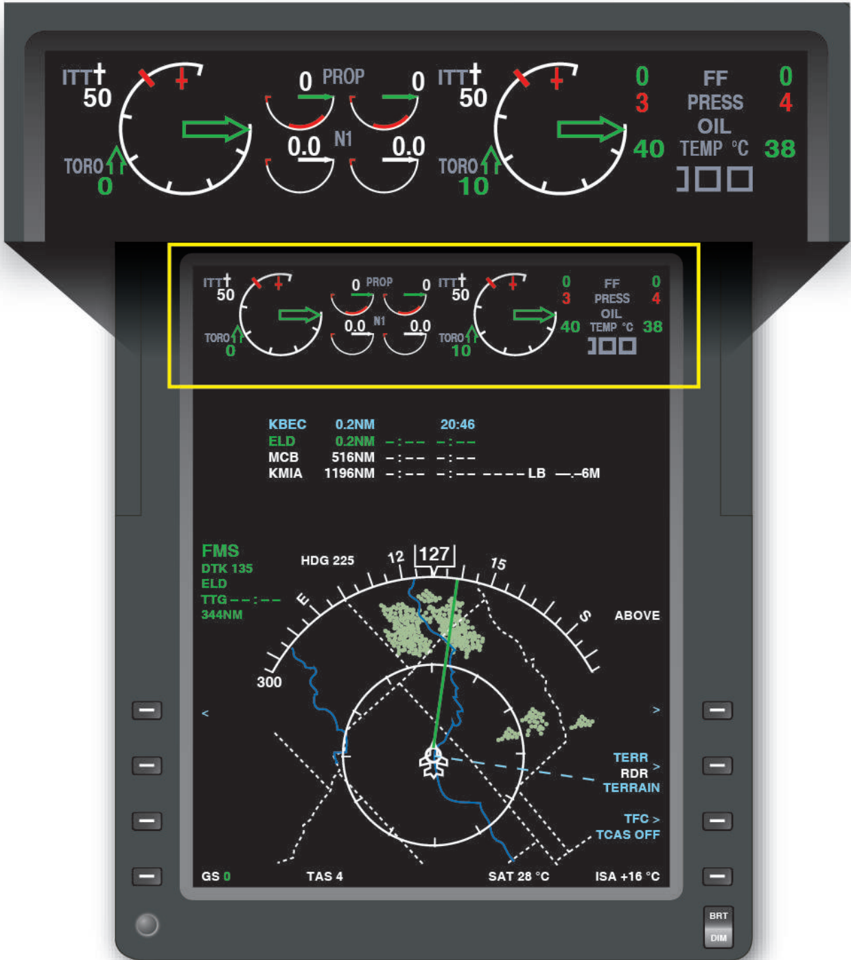
Figure 15-7. Engine instruments—split shaft/free turbine engine.
