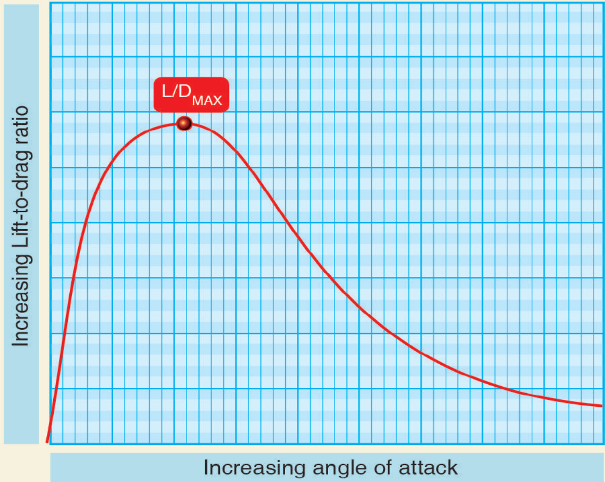
Figure 3-23. L/D_{MAX} .
