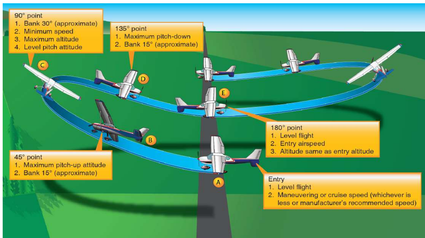
Figure 10-4. Lazy eight.
