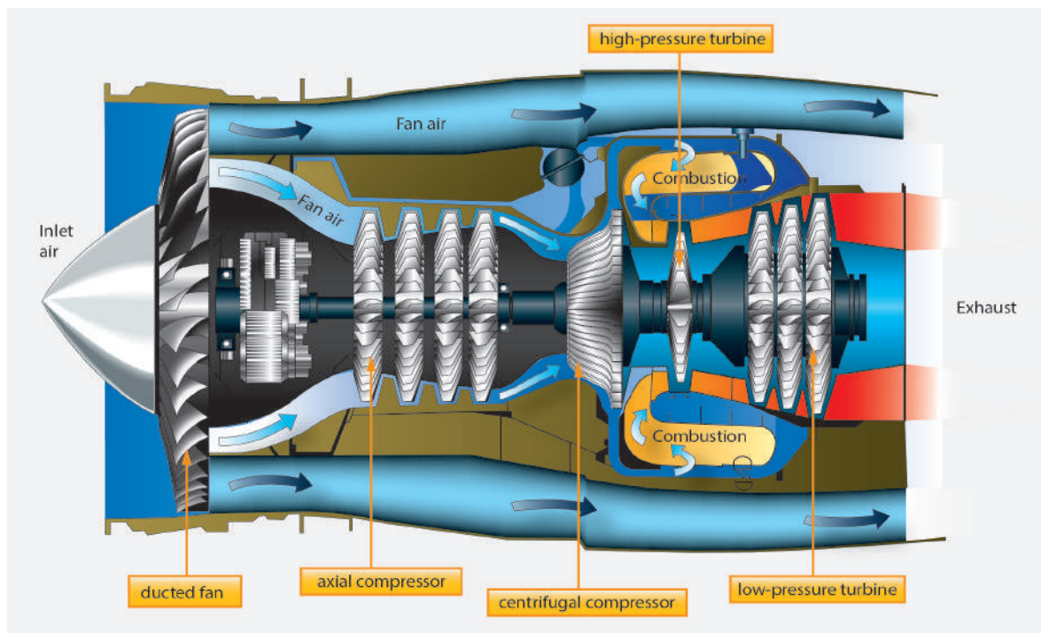
Figure 16-2. Turbofan engine.
